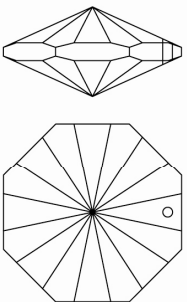
Art. 1080, Size: 14, 16, 18, 20, 22, 24, 26, 28, 30 mm.
