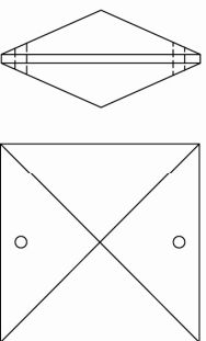
Art. 2020, Size: 16, 18, 20, 22, 24, 26, 28 mm.
